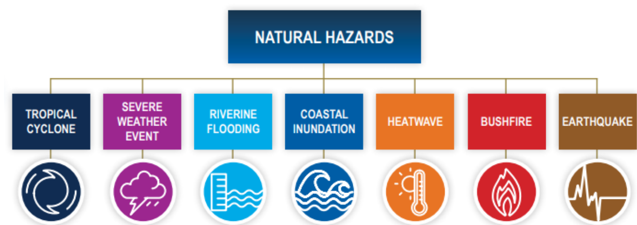
Figure 28 – Natural hazards.
