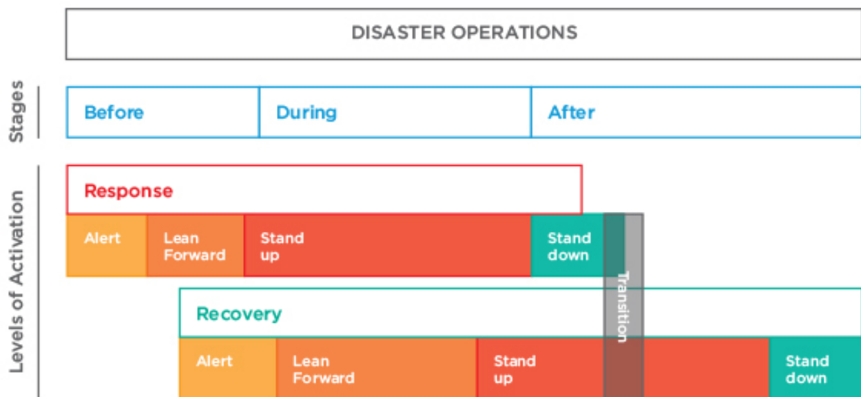
Figure 6 – Disaster operations.
