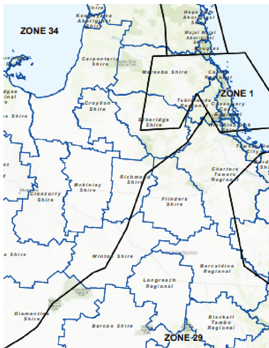
Figure 60 – Earthquake zones.
